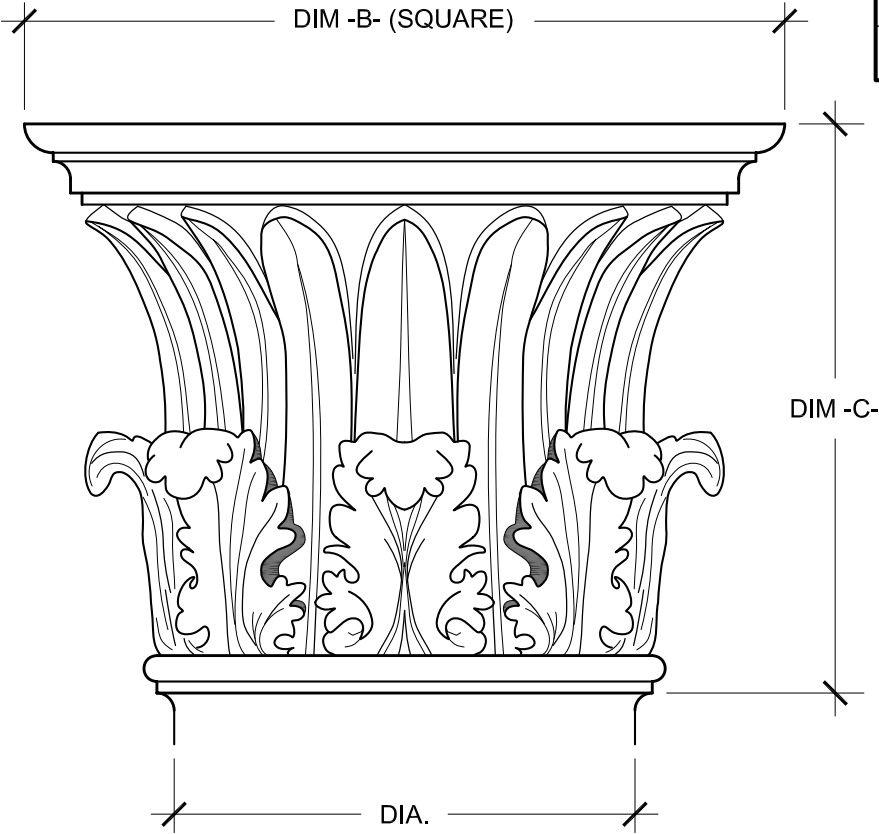
SIDE VIEW
